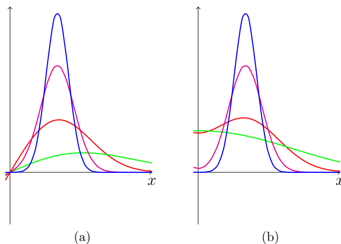
Figure 3.1: Plots of G_D(x, y, t) and G_N(x, y, t) as y \rightarrow 0 (for some values of t )
