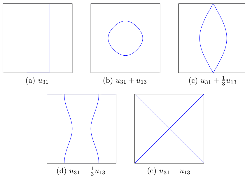
Figure 13.5: \lambda = 10
