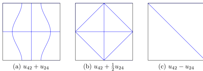
Figure 13.8: \lambda = 20
