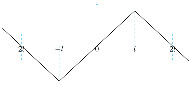
(b) f(0) = 0
