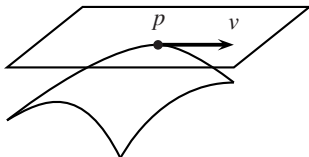
Fig. 2.2. A tangent vector v to a surface at p .
