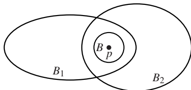
Fig. A.3. Criterion for a basis.
