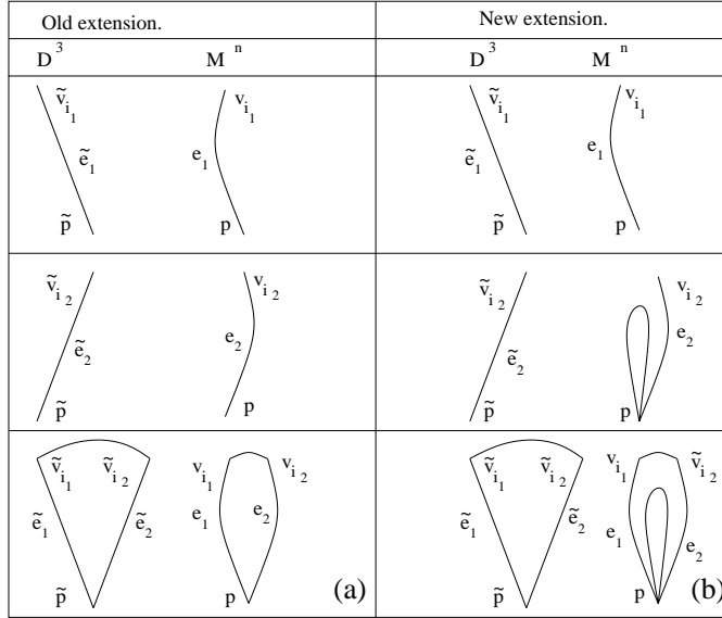
Figure 2: Modified extension.
