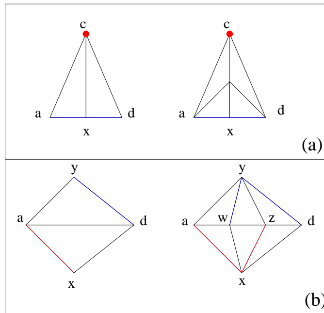
Figure 4: Simplicial subdivisions
