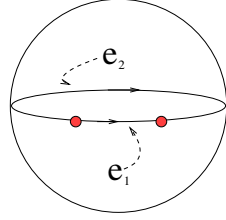
Figure 1: Short geodesic segments on a round sphere.
