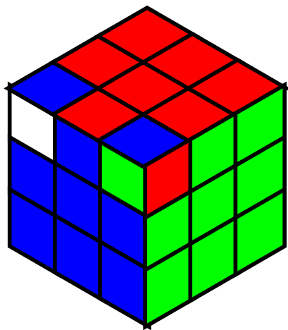
Figure 5: Effect Of R^{-1}DRFDF^{-1}U^{-1}FD^{-1}F^{-1}R^{-1}D^{-1}RU
