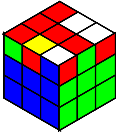
Figure 2: Effect Of The Move BULU^{-1}L^{-1}B^{-1} . (But We Want To Use BLUL^{-1}U^{-1}B^{-1} Here)
