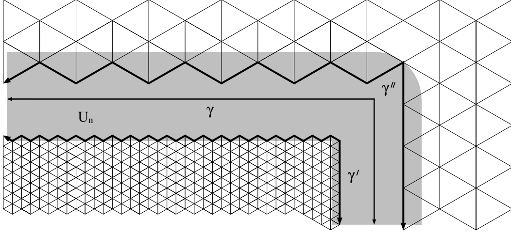
FIGURE 14. The shaded region represents part of U_n of \Gamma_n . The region interior to U_n is covered by a Euclidean equilateral triangulation with side lengths \epsilon_{n+1} (the small triangles). The “exterior” region covered by elements of the triangulation \mathcal{T}_{n-1} constructed at the previous stage (drawn here as larger equilateral triangles, but they need not be Euclidean triangles, only conformal images of such). The results of the previous section are used to triangulate the intervening region with the given boundary vertices, and then a quasiconformal correction will be applied to obtain an equilateral triangulation of the sphere. The correction map is conformal off U_n , and has derivative \approx 1 at points more than \frac{1}{2} \cdot 16^{-n} from U_n .
