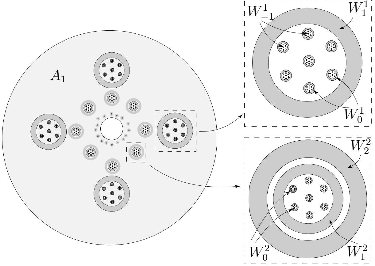
FIGURE 9. Illustrated is the covering \mathcal{C}_1 , and the notation W_k^n for elements of \mathcal{C}_1 (see Notation 8.3). The elements of \mathcal{C}_m for m > 1 are obtained by essentially placing a scaled-down copy of \mathcal{C}_{m-1} in each annulus in the covering \mathcal{C}_{m-1} .
