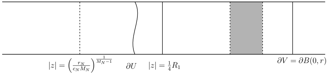
FIGURE 5. A schematic for Definition 5.4 and Lemma 5.5. The critical points for q_N lie on the circle |z| = \left( \frac{r_N}{c_N M_N} \right)^{\frac{1}{M_N-1}} , and the associated critical values lie in an annulus contained in V , illustrated in gray. So U contains the critical points of q_N , and it will also be verified that U \subset D .
