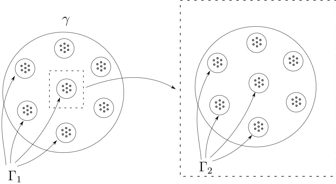
FIGURE 6. Illustrated is Definition 5.8 of the families \Gamma_n .
