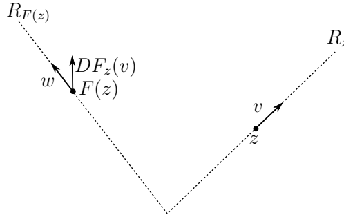
FIGURE 11. A schematic for the statement of Lemma 9.3.
