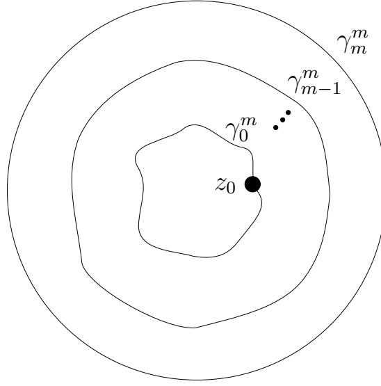
FIGURE 15. Illustrated is a brief sketch of the curves \gamma_k^m for 0 \leq k \leq m .
