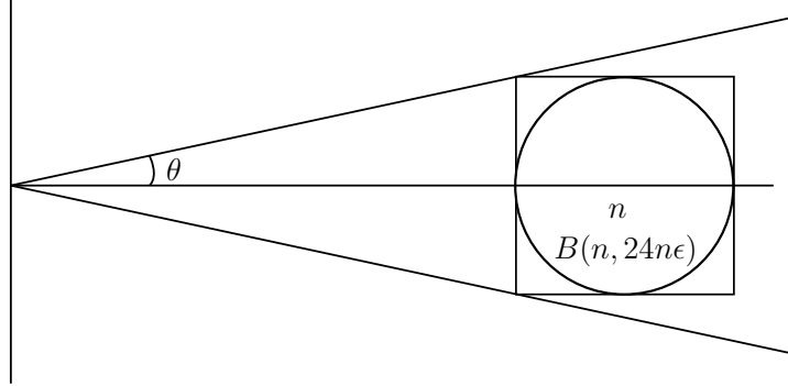
FIGURE 12. A schematic for the proof of Lemma 9.4.
