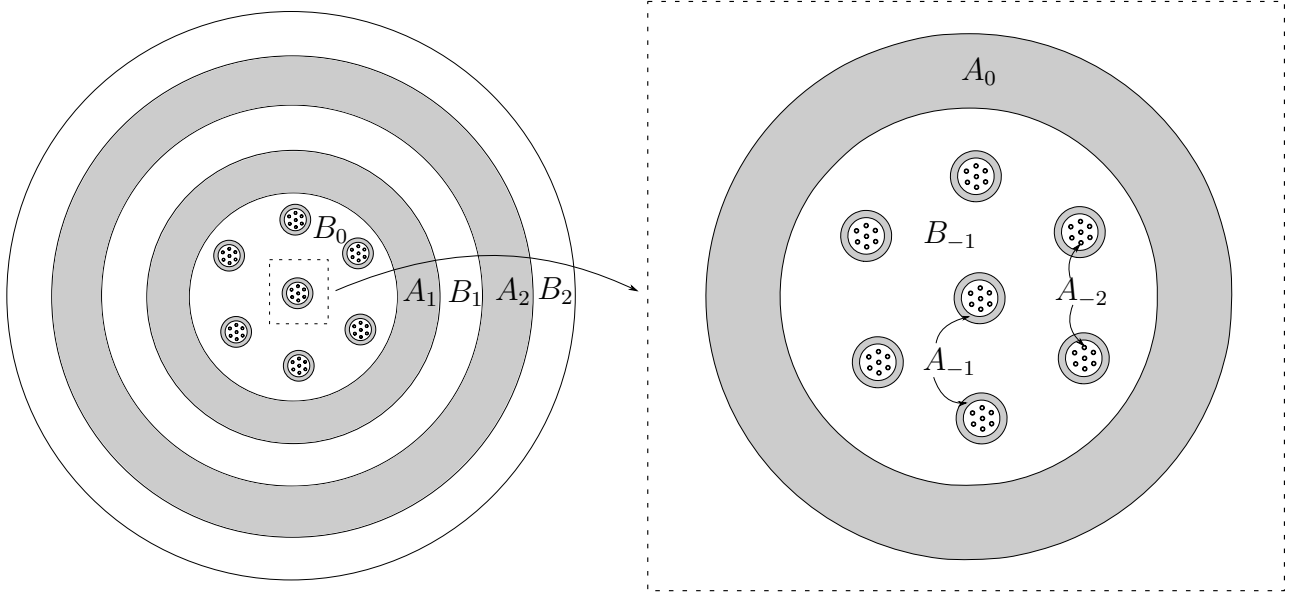
FIGURE 8. Illustrated is Definition 7.1 of A_k, B_k for negative k . Each connected component of A_0 maps conformally onto A_1 ; therefore, each connected component of A_0 contains 2^N many connected components of A_{-1} . The picture repeats itself as we zoom in. The set B_0 is the region between the outer boundaries of the components of A_0 and the inner boundary of A_1 .
