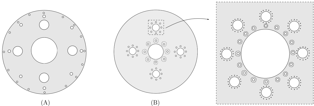
FIGURE 1. (A) and (B) illustrate the concept of infinite outer-connectivity, and infinite inner-connectivity, respectively. (A) and (B) also accurately describe the topology of the m.c.w.d.'s in [Bis18] and Theorem 1.1, respectively. As seen, the structure in (B) is more intricate.
