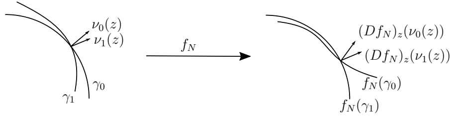
FIGURE 13. A schematic for the proof of Lemma 9.8 in the key step of m = 1 and n = 0 . In this case, \gamma_0 and f_N(\gamma_1) are circles, and (Df_N) : T_z\mathbb{C} \rightarrow T_{f_N(z)}\mathbb{C} maps the outward pointing normal \nu_1(z) to \gamma_1 to an outward pointing normal (Df_N)_z(\nu_1(z)) of the circle f_N(\gamma_1) . This allows us to apply Lemma 9.4 to estimate the angle between (Df_N)_z(\nu_1(z)) and (Df_N)_z(\nu_0(z)) , which coincides with the angle between \nu_1(z) and \nu_0(z) .
