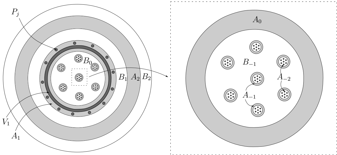
FIGURE 2. This Figure illustrates the definition of A_k, B_k for all k \in \mathbb{Z} . The annuli A_k are shaded light grey, and the B_k are white. Also shown is V_1 \subset A_1 and the “petals” P_j \subset A_1 (in dark grey).
