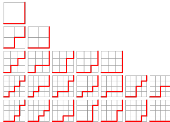
Figure 1: all Dyck paths up to n = 4
