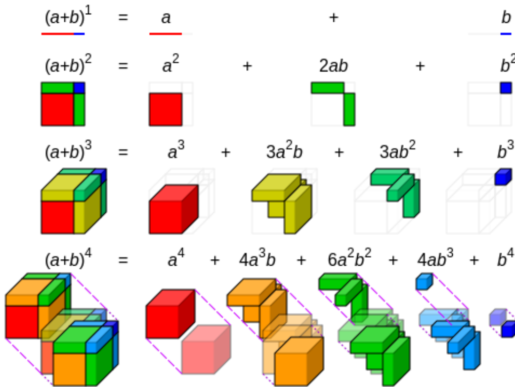
Figure 2: Visualization of the binomial theorem
