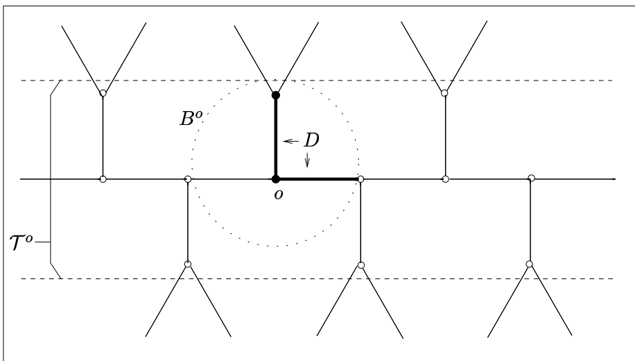
FIGURE 7. A fundamental domain (in bold) D in the fixed point set of the compact non-elliptic element \gamma \in GL_2 of Example 2.5.
