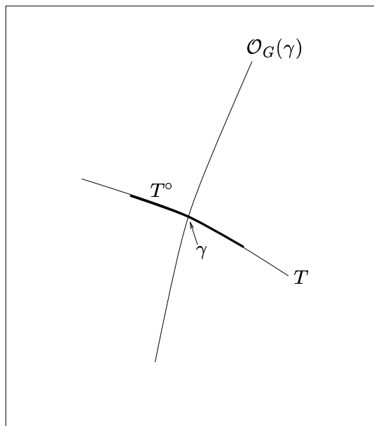
FIGURE 6. Local picture around \gamma
