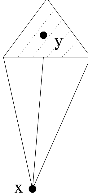
Figure 2: (m, r) -umbrella
