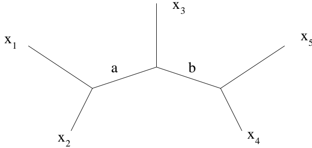
Figure 7. A rational curve with 5 marked points.
