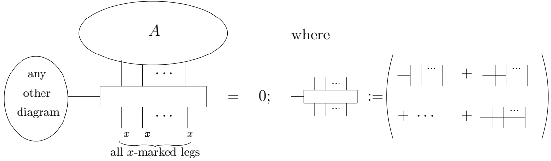
Figure 1. Invariance with respect to x of a diagram A .
