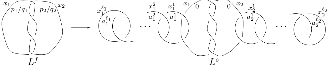
Figure 2. The link L^s is obtained from L by changing all the framings p_i/q_i to 0 and shackling all the components x_1, \dots, x_n with Hopf chains marked x_1^1, \dots, x_1^{\ell_1}, \dots, x_n^1, \dots, x_n^{\ell_n} and framed a_1^1, \dots, a_1^{\ell_1}, \dots, a_n^1, \dots, a_n^{\ell_n} , so that p_i/q_i = \langle a_i^1, \dots, a_i^{\ell_i} \rangle as in Equation (6).
