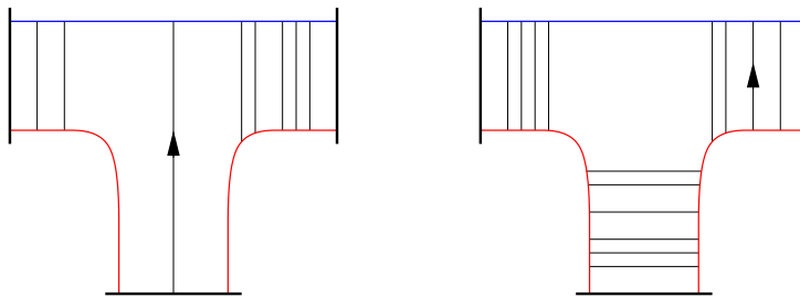
Figure 3.1: The lower and the vertical sides of R lie in \partial S : the longer boundary arcs lie in A_\ell . The arcs in the interior are subarcs of \omega . The arc with the arrow is \delta_1 on the left and is \delta_m on the right.
