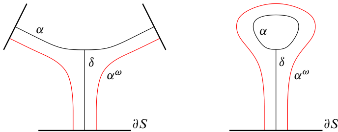
Figure 2.1: The result of surgery, \alpha^\omega , is either a pair of arcs or a single arc as \alpha is an arc or a curve.
